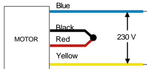
Dual Voltage Wiring Diagram 230VAC
