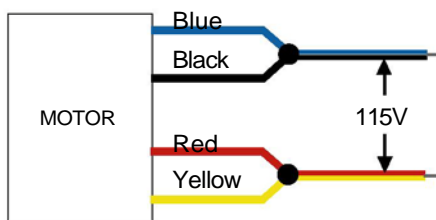
Dual Voltage Wiring Diagram 115VAC
